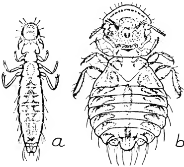
Fig. 59. a, Variable hen louse, Lipeurus caponis (L.) (Ohio Agr. Expt. Sta.); b, Large chicken louse, Gonicocotes gigas (Taschenberg) (Ohio Expt. Sta.).
